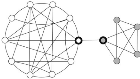
Fig. 10 – A two-cluster graph. If a blind random walk is currently in the white thick-bordered vertex, it will remain in the white cluster with probability \frac{5}{6} and switch over to the grey cluster with probability \frac{1}{6} . Being at any other white vertex, a random walk will necessarily stay within the white cluster. Similarly, a blind random walk on the grey thick-bordered vertex has probability \frac{1}{4} to switch over to the white cluster, and probability \frac{3}{4} to remain in the grey cluster.
